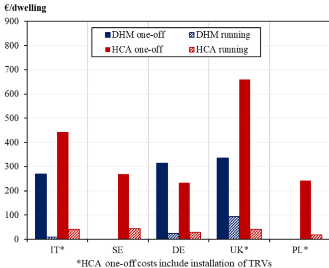
Fig. 6. Total one-off and running costs of DHMs and HCAs installation per dwelling.
